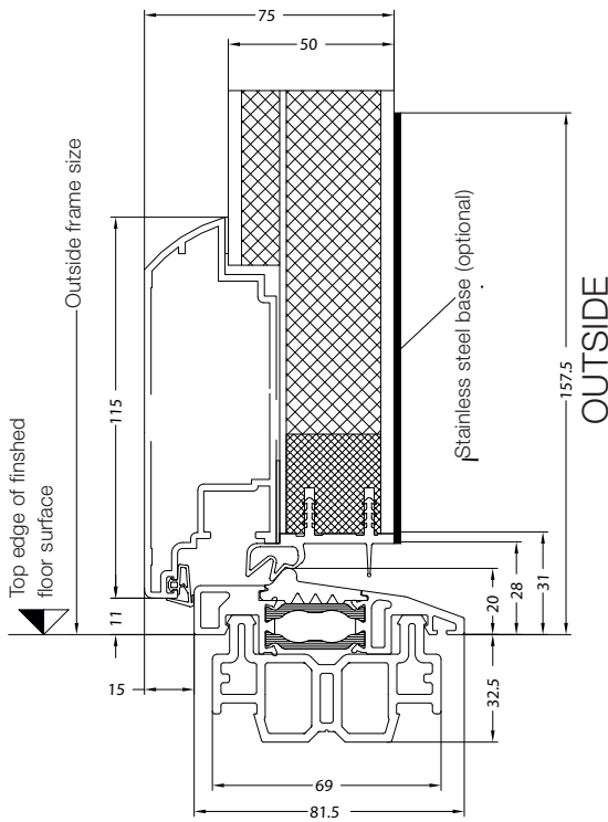
Vertical section (floor connection)
